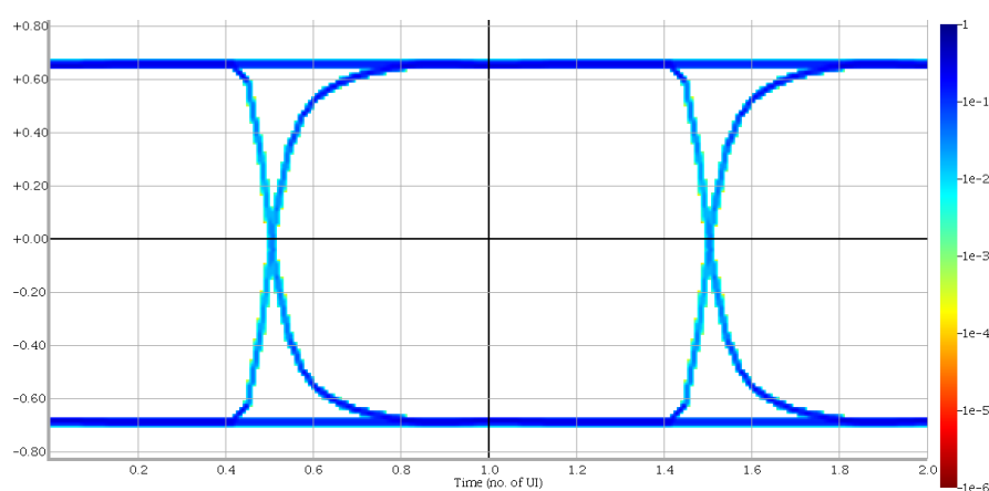
Name: RX_IN_PT2 Height:1.321 Width:0.977 Jitter:0.023
