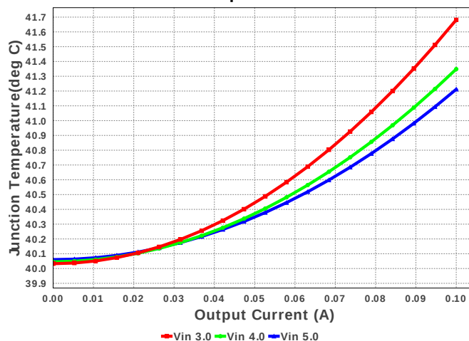
Junction Temperature vs Iout
