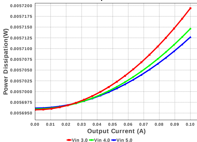
IC Power dissipation vs Iout
