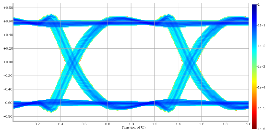
Name: SC_OUT_PT2 Height:1.12 Width:0.859 Jitter:0.141
