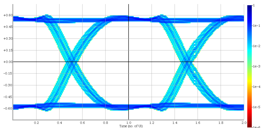
Name: OUT_PT2 Height:1.075 Width:0.859 Jitter:0.141
