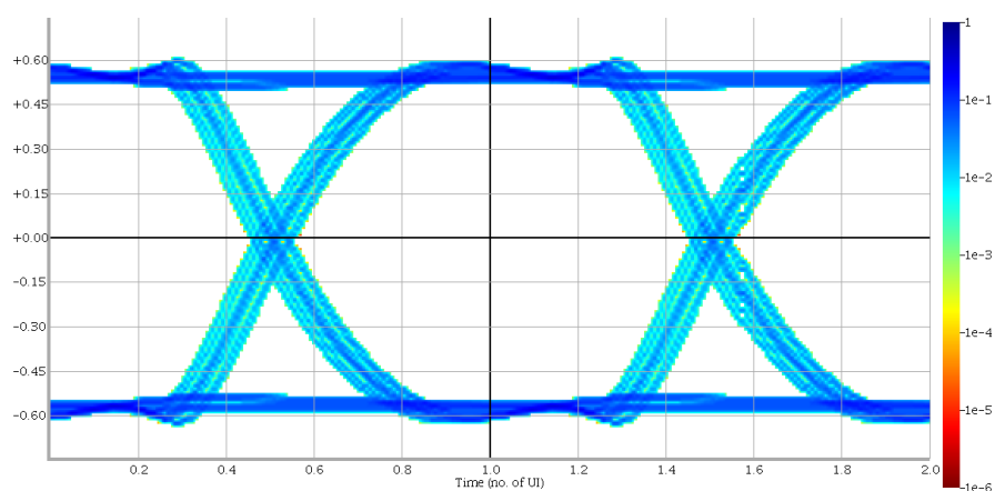
Name: RX_IN_PT2 Height:1.075 Width:0.859 Jitter:0.141
